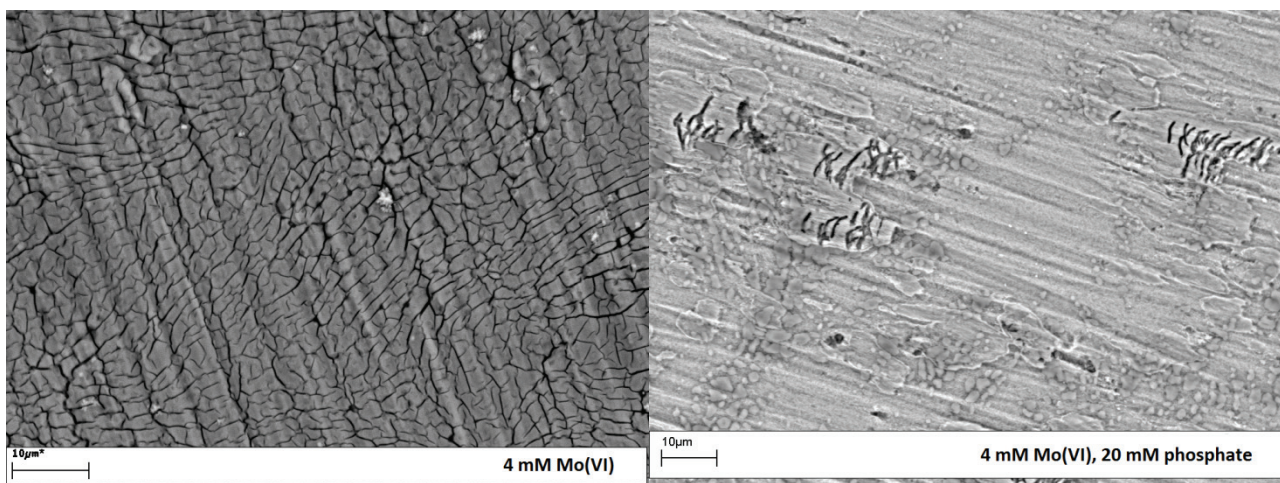
Figure 5. SEM images on Ti-RDEs polarized for 30 min at -3 \text{ kA m}^{-2} in 2 M NaCl, 4 mM Mo(VI), \text{pH}\approx 6.5 and 70^\circ\text{C} with and without 20 mM phosphate. The rotation rate during polarization was 3000 rpm.
