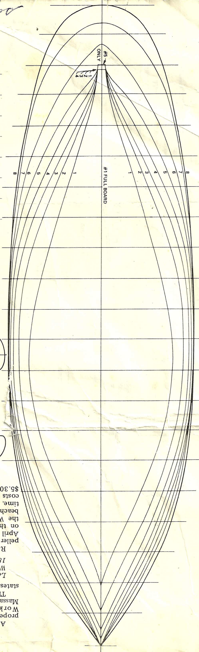
PROPELLER BLADE As traced from Weymouth Iron Works Pattern Drawing - 1881
