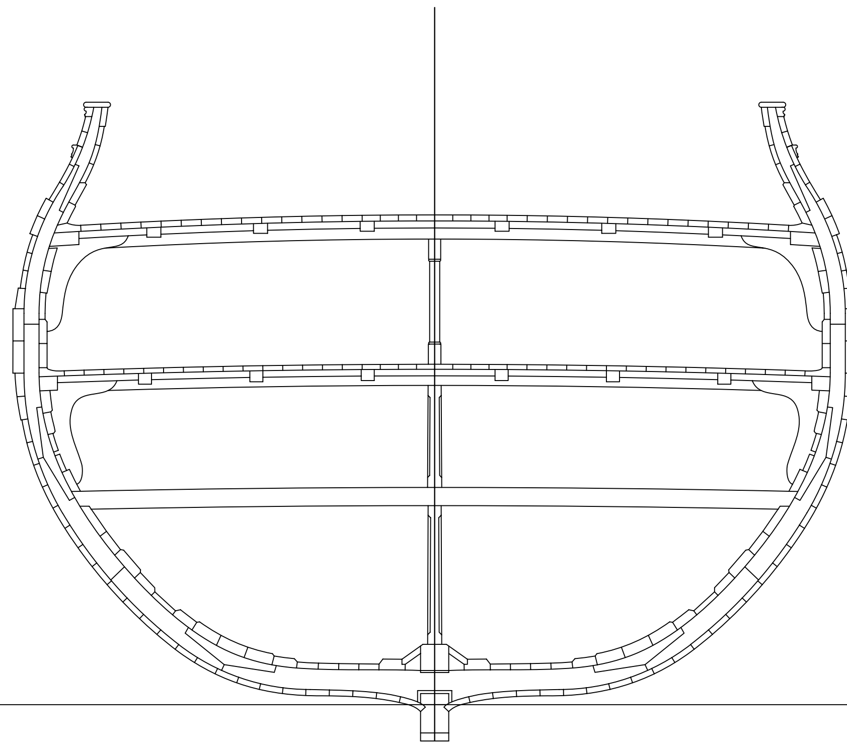
MIDSHIP SECTION
