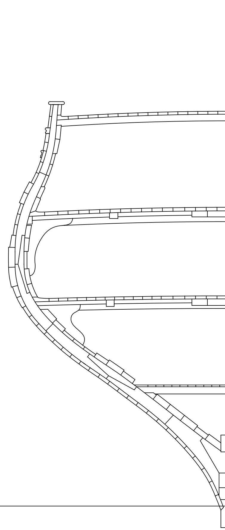
SECTION 17 (LOOKING AFT)
