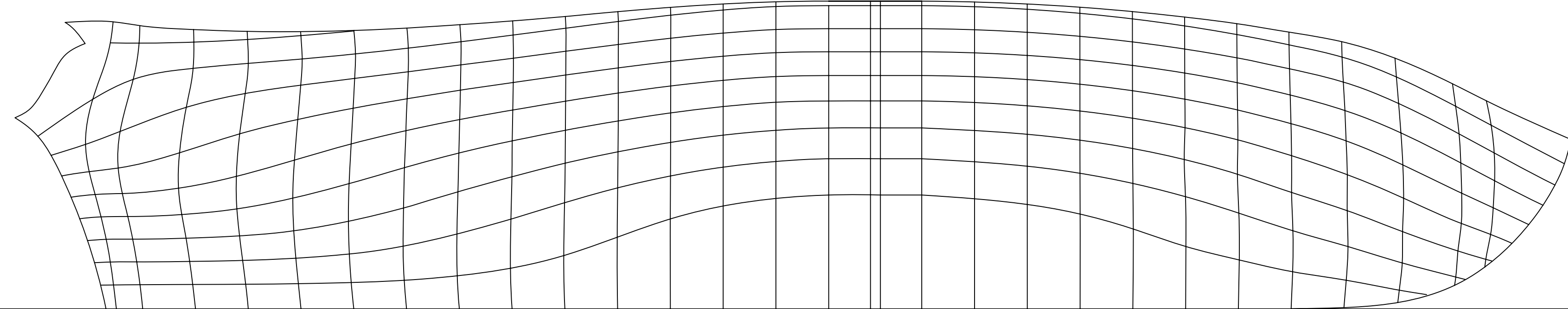
EXPANDED NET OF SECTIONS AND WATERLINES
