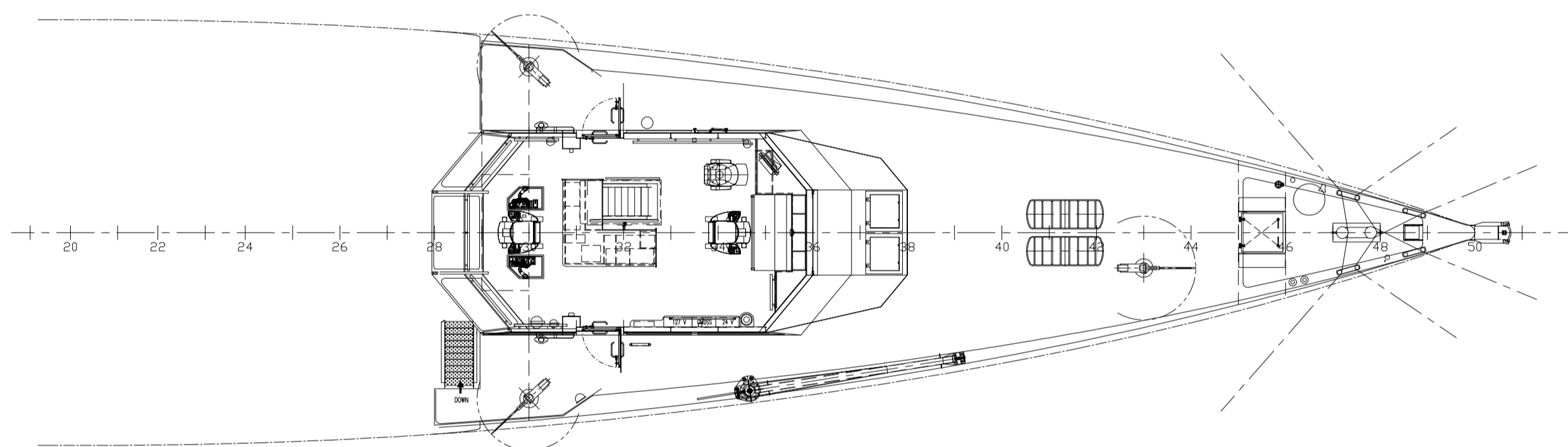
Bridge Deck
